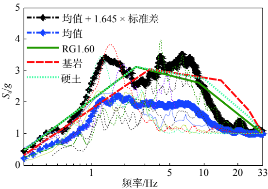
图 5 输入地震动标准化 5% 阻尼比加速度反应谱 Fig. 5 Normalized acceleration response spectrum of selected ground motions considering 5% damping ratio
